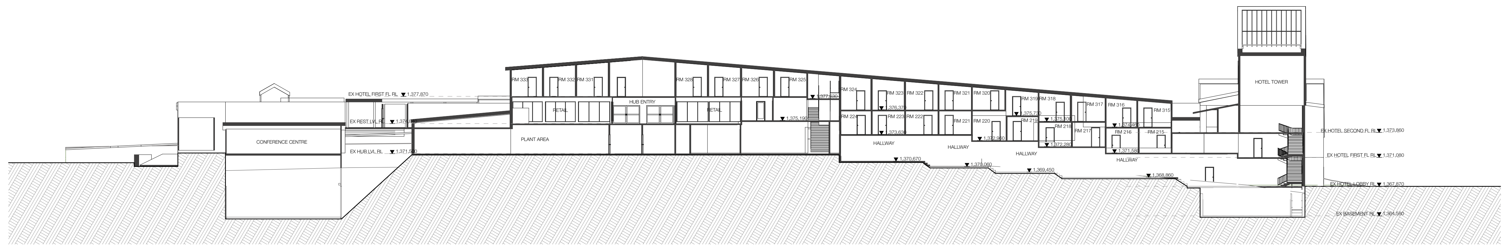
1 LONG SECTION HOTEL / TOWER 1:250
