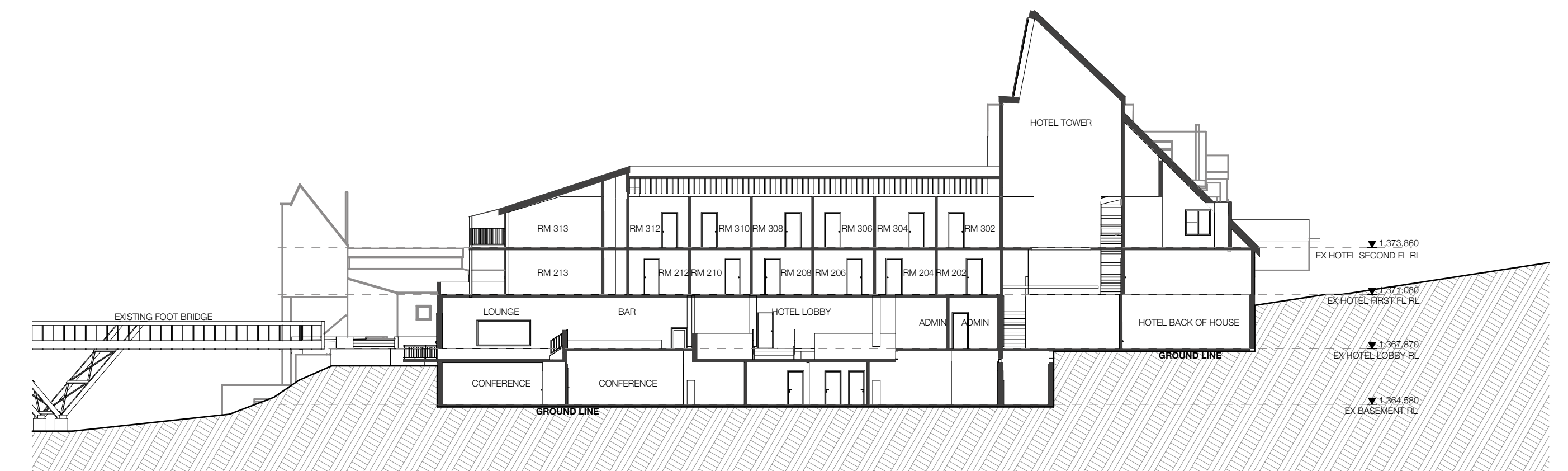
6 HOTEL WEST WING SECTION 1:250
