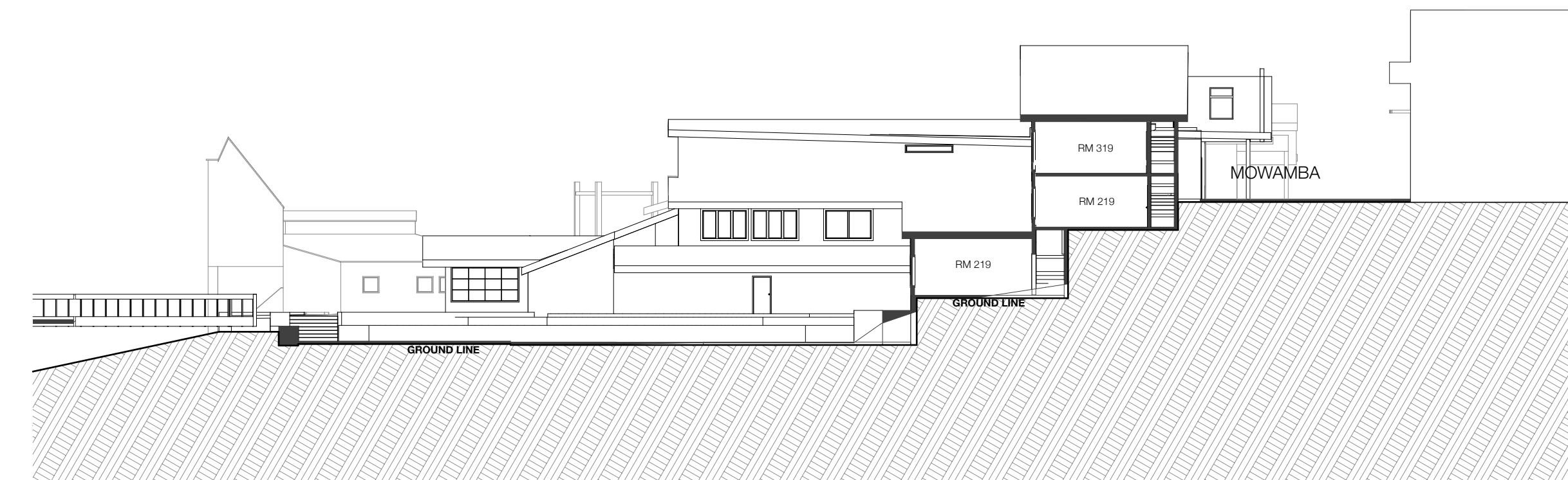
3 COURTYARD EAST SECTION 1:250
