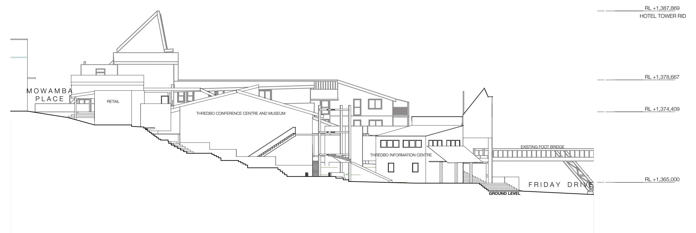
4 EAST ELEVATION 1:250
