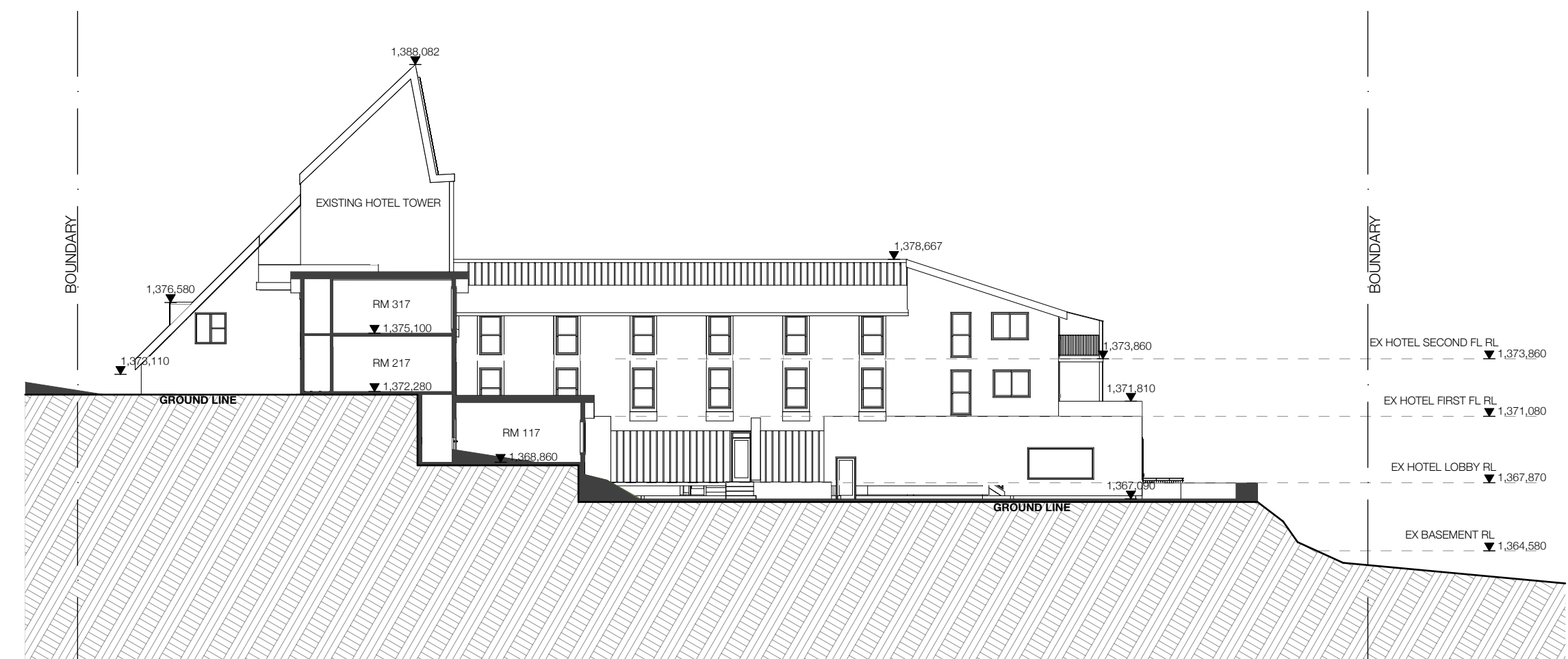
4 COURTYARD WEST SECTION 1:250
