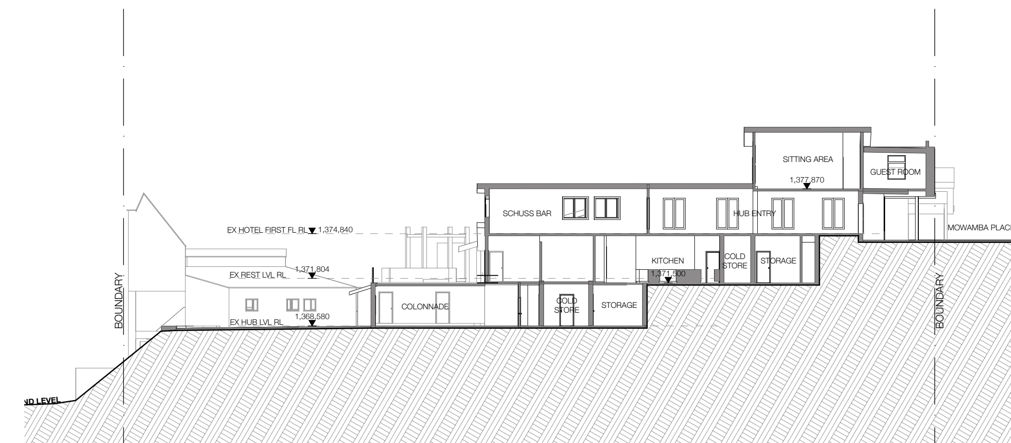
5 CENTRAL STAIR SECTION 1:250
