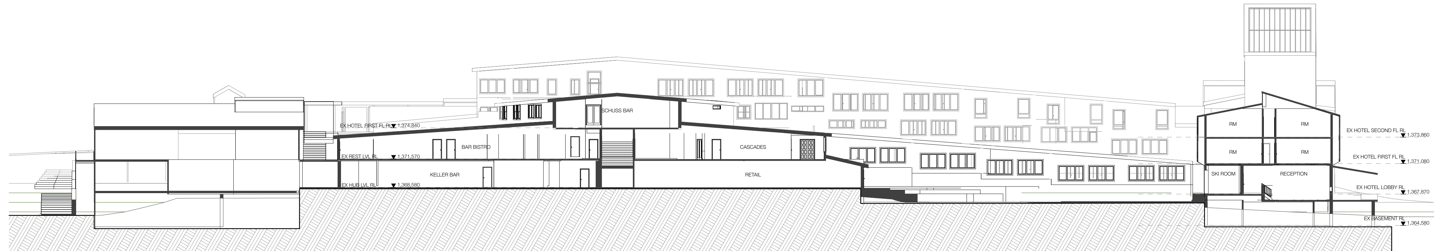
2 LONG SECTION RESTAURANTS / COURTYARD 1:250
